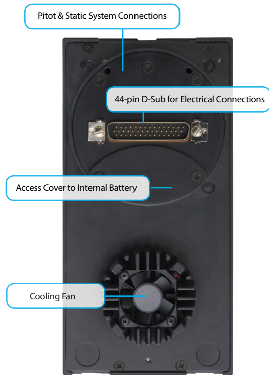
Figure 1-6 EFD1000 Pro MAX Display Unit Rear Connections
